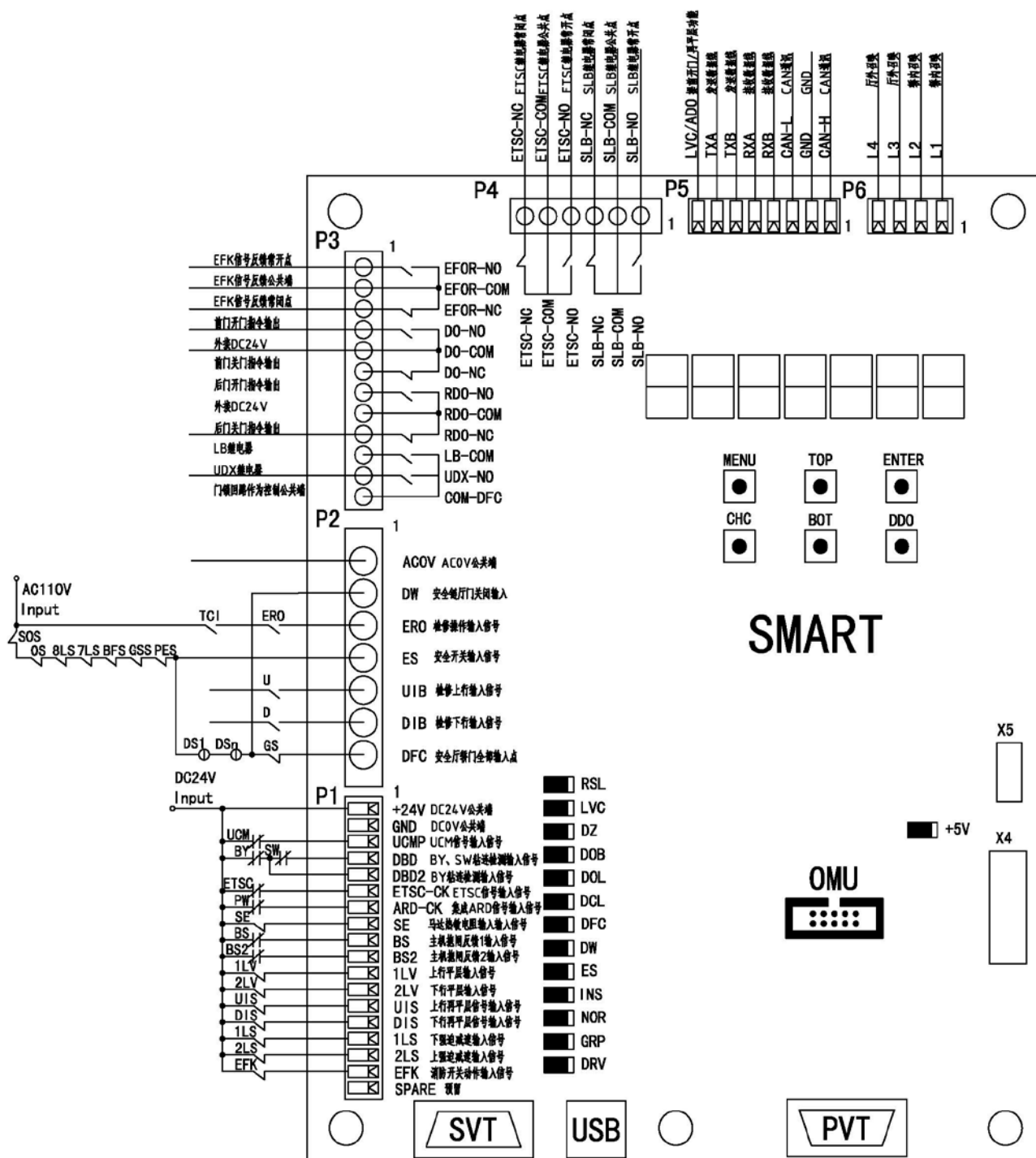
External Wiring Diagram
